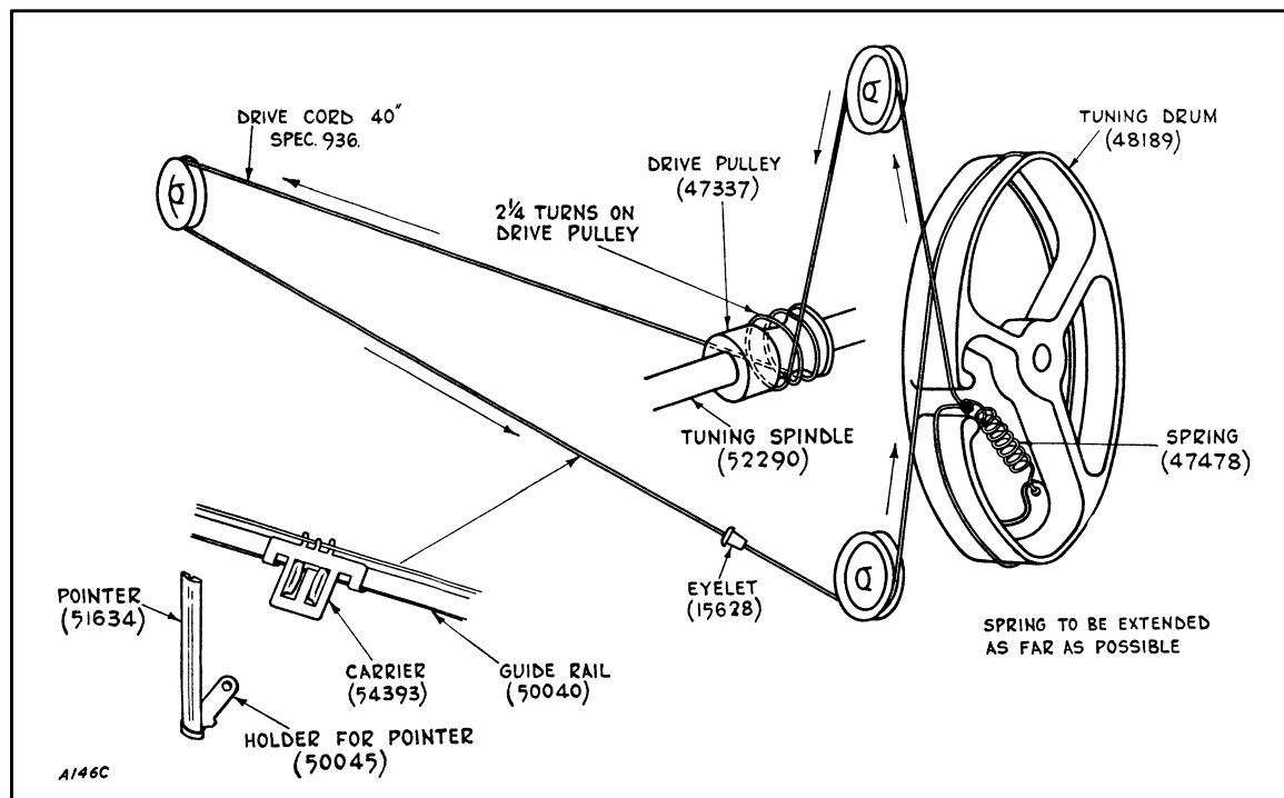
Fig. 5. The cord drive
