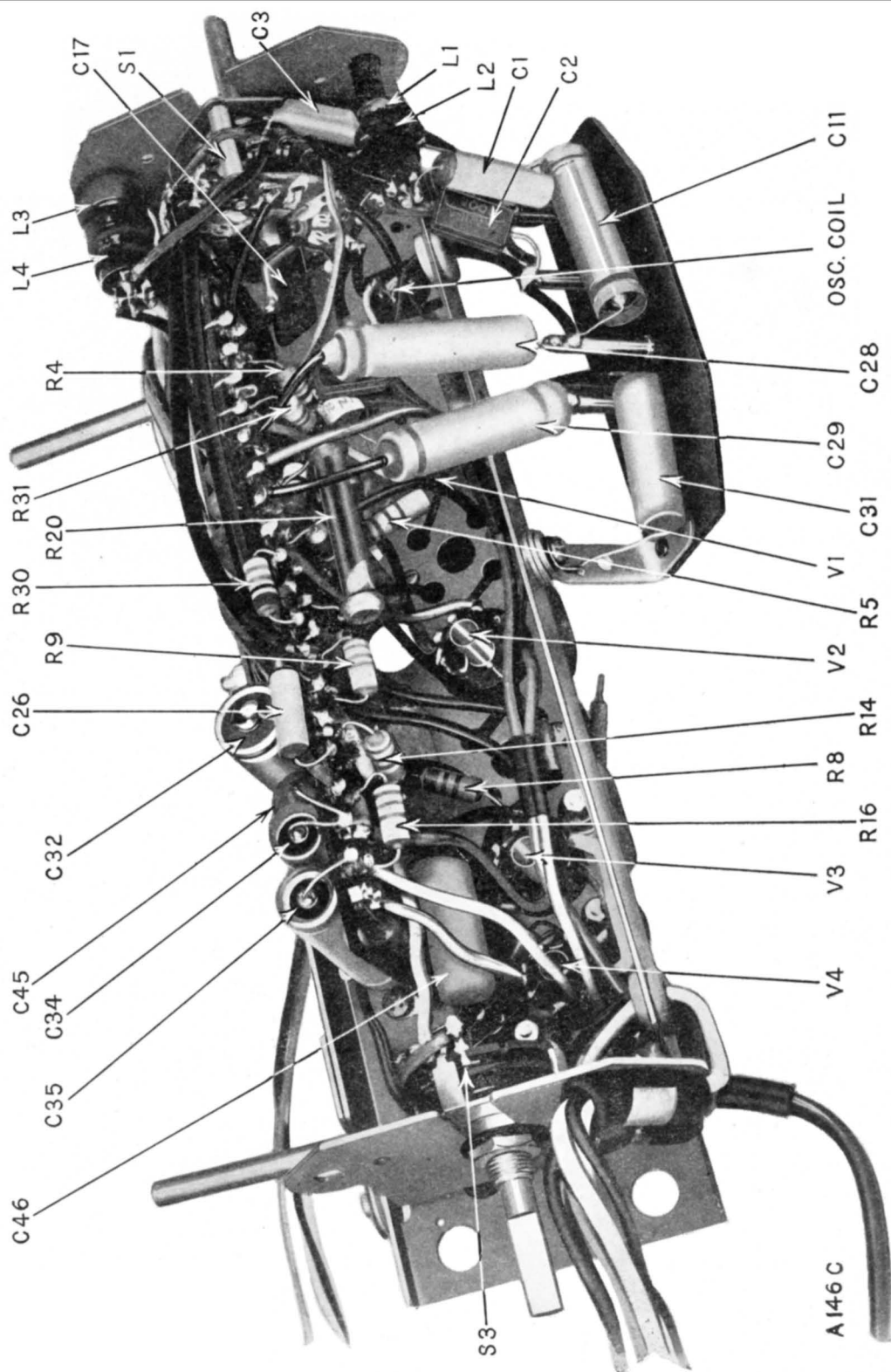
Fig. 6. Underneath view of the Receiver Chassis. The top view is on page 12.
