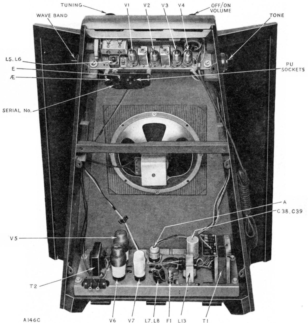
Fig. 1. Rear view of the complete receiver
